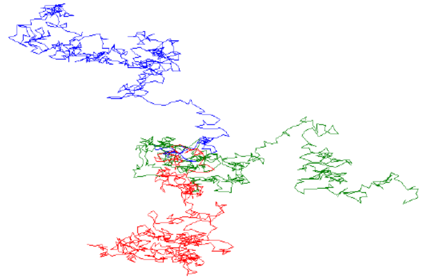
Three random walks originating from a common starting point.
